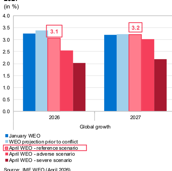
Chart V.0.1 Global growth projections for 2026 and 2027 (in %)
