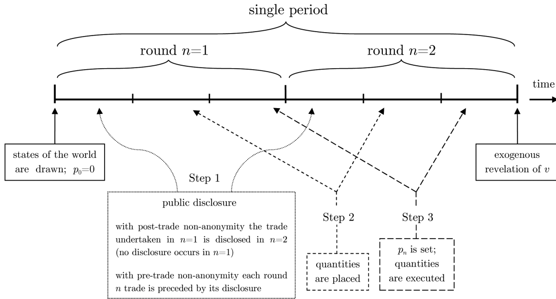
Fig. 1. Timing of events in the single period.
